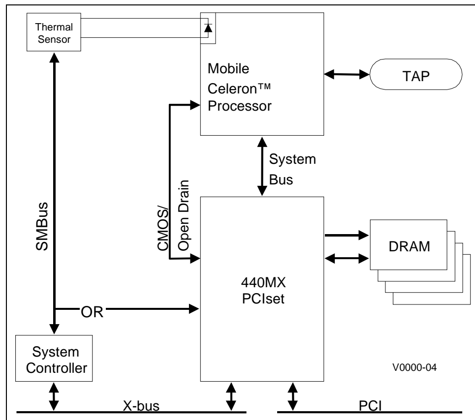
Figure 1. Signal Groups of a Mobile Celeron Processor-Based System
