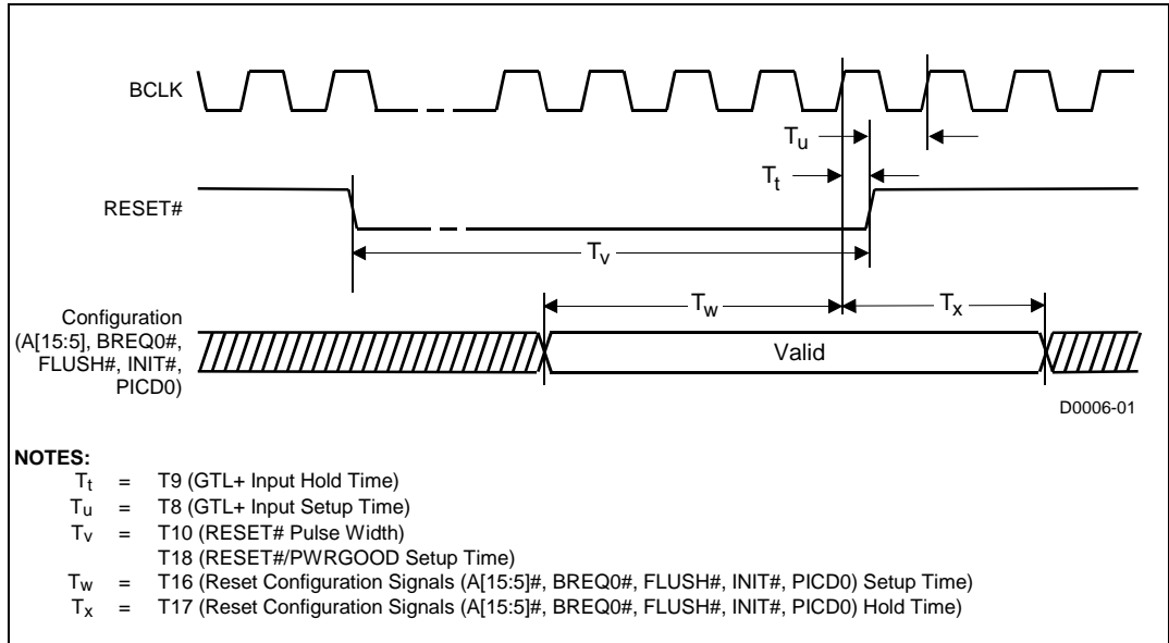
Figure 10. Power-on Reset Timings
