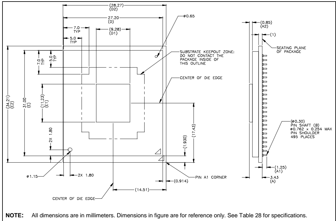
Figure 21. Socketable Micro-PGA2 Package - Top and Side View
