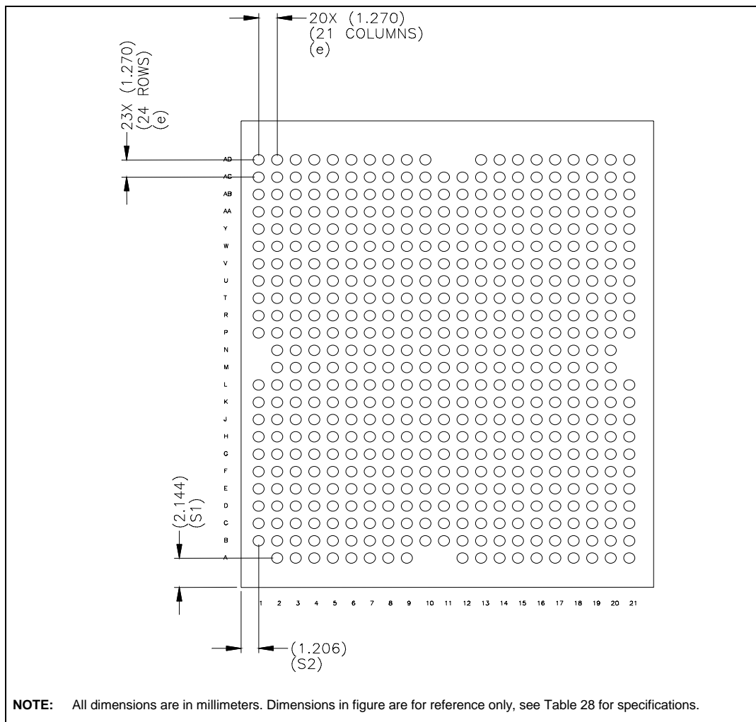
Figure 22. Socketable Micro-PGA2 Package - Bottom View
