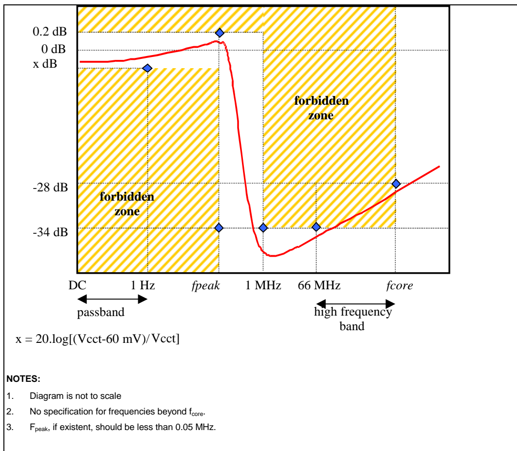
Figure 25. PLL Filter Specifications
