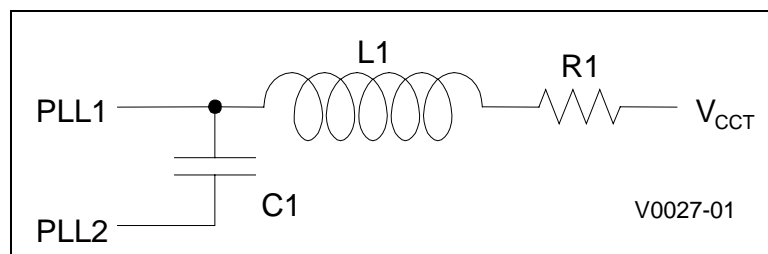
Figure 4. PLL RLC Filter
