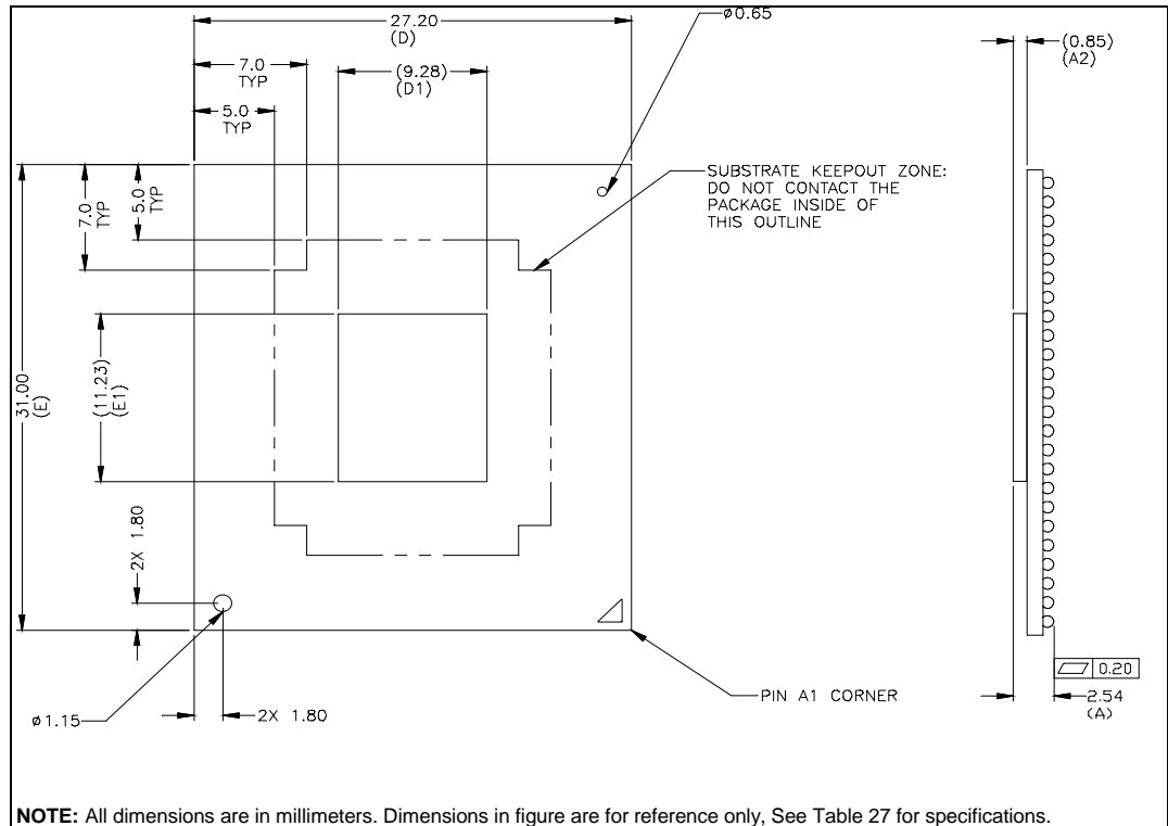
Figure 19. Surface-mount BGA2 Package - Top and Side View
