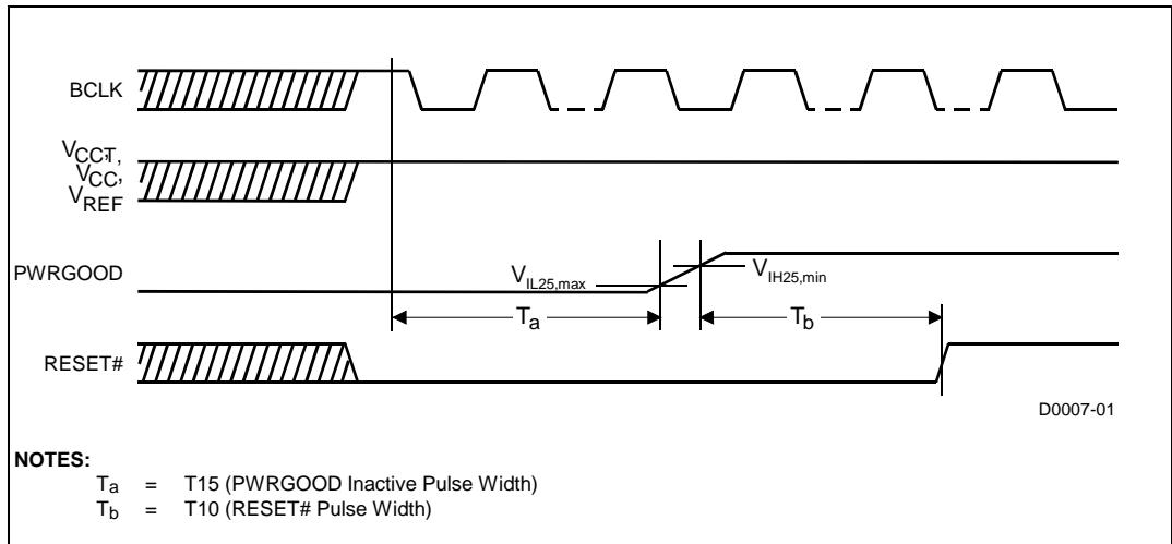
Figure 10. Power-on Reset Timings
