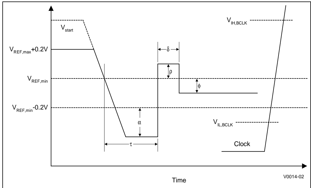
Figure 17. High to Low, GTL+ Receiver Ringback Tolerance
