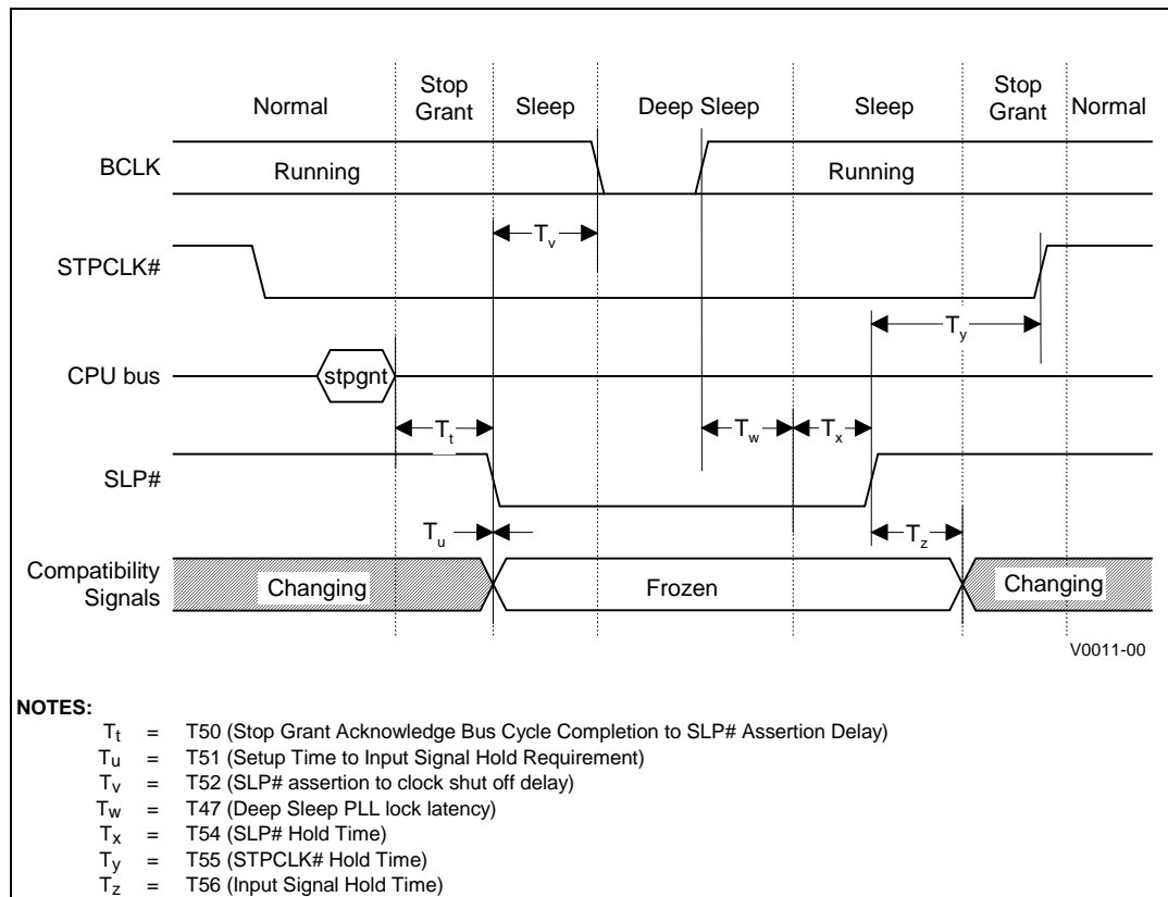
Figure 14. Stop Grant/Sleep/Deep Sleep Timing
