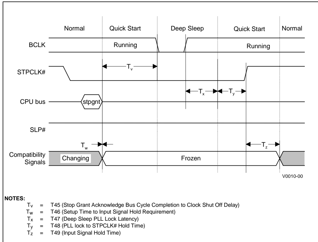
Figure 13. Quick Start/Deep Sleep Timing
